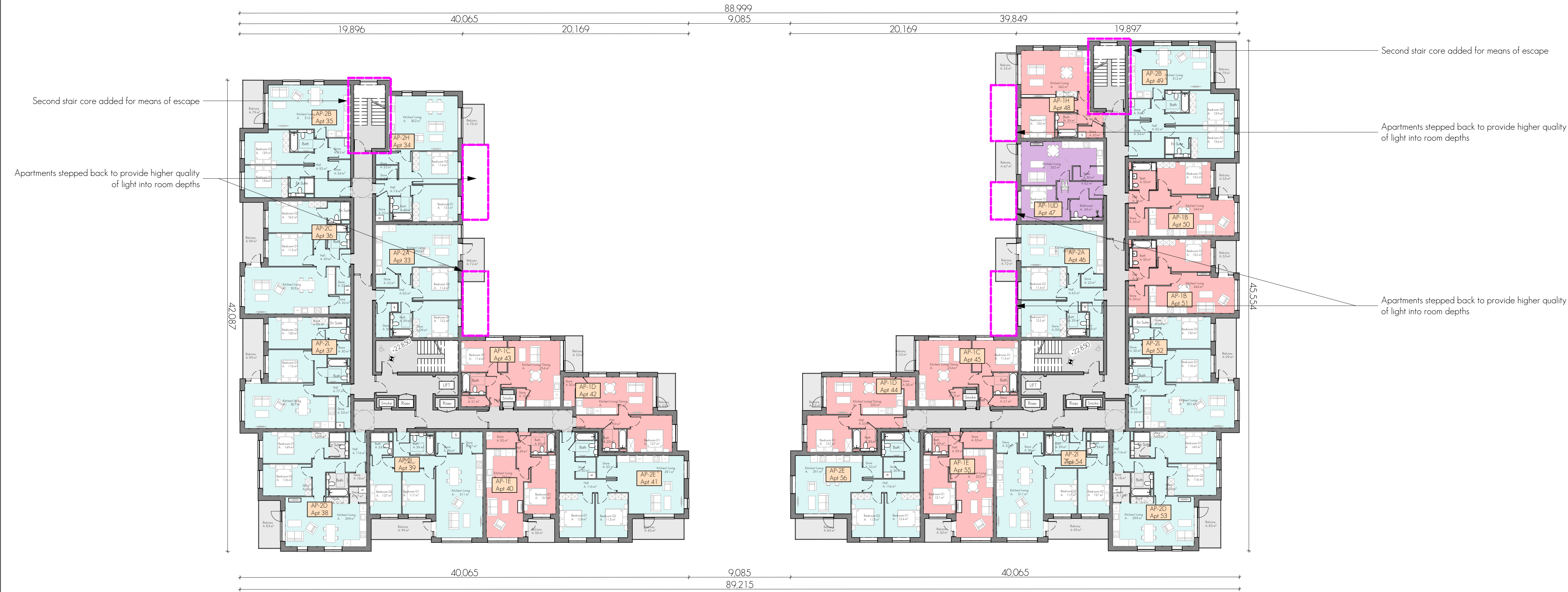
First Floor Plan 1:200
